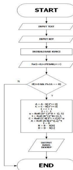
Gbr 11 Diagram Alur Algoritma Dekripsi RC6
