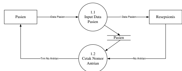
Gambar 3 Diagram 1.1
