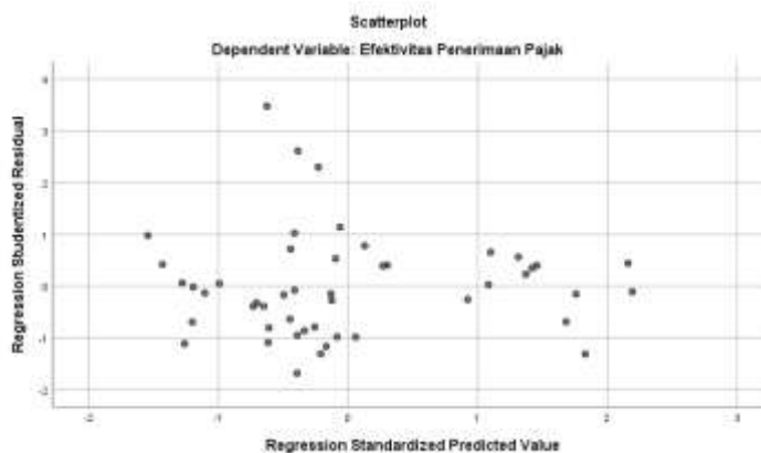
Gambar 2. Diagram Scatterplot
