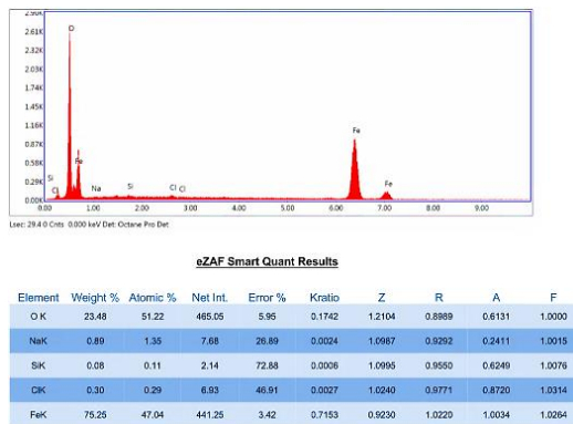
b) Logam tanpa inhibitor korosi (0 ppm)
