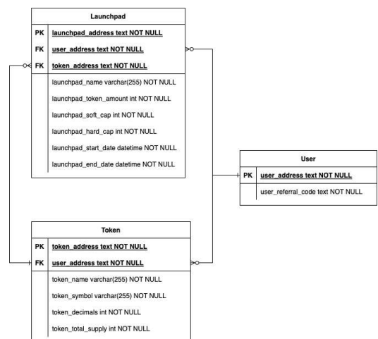
Gambar 4. Database Design
