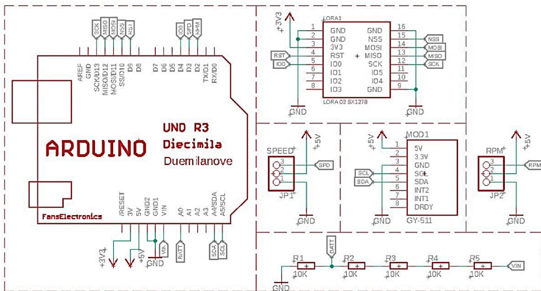
Fig. 3. Wiring diagram of electricity design
