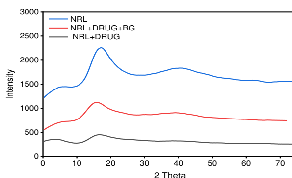
Figure 4. XRD spectrum o XRD spectra of biomembranes.
