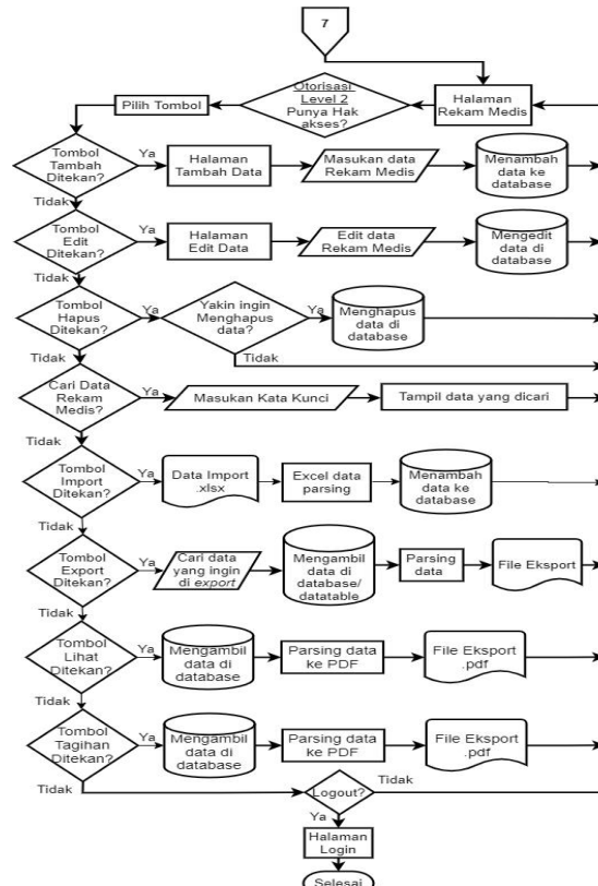
Gambar 2. 8 Flowchart Rekam Medis
