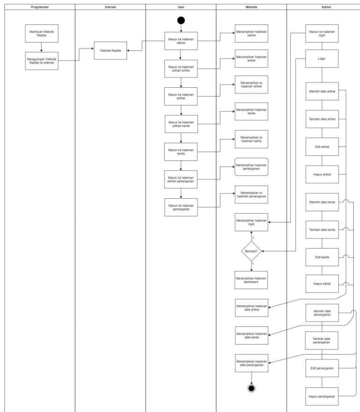
Gambar 4. Activity Diagram
