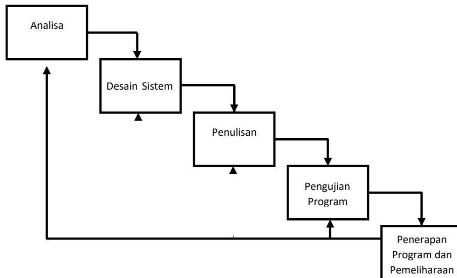
Gambar 1. Metode Waterfall
