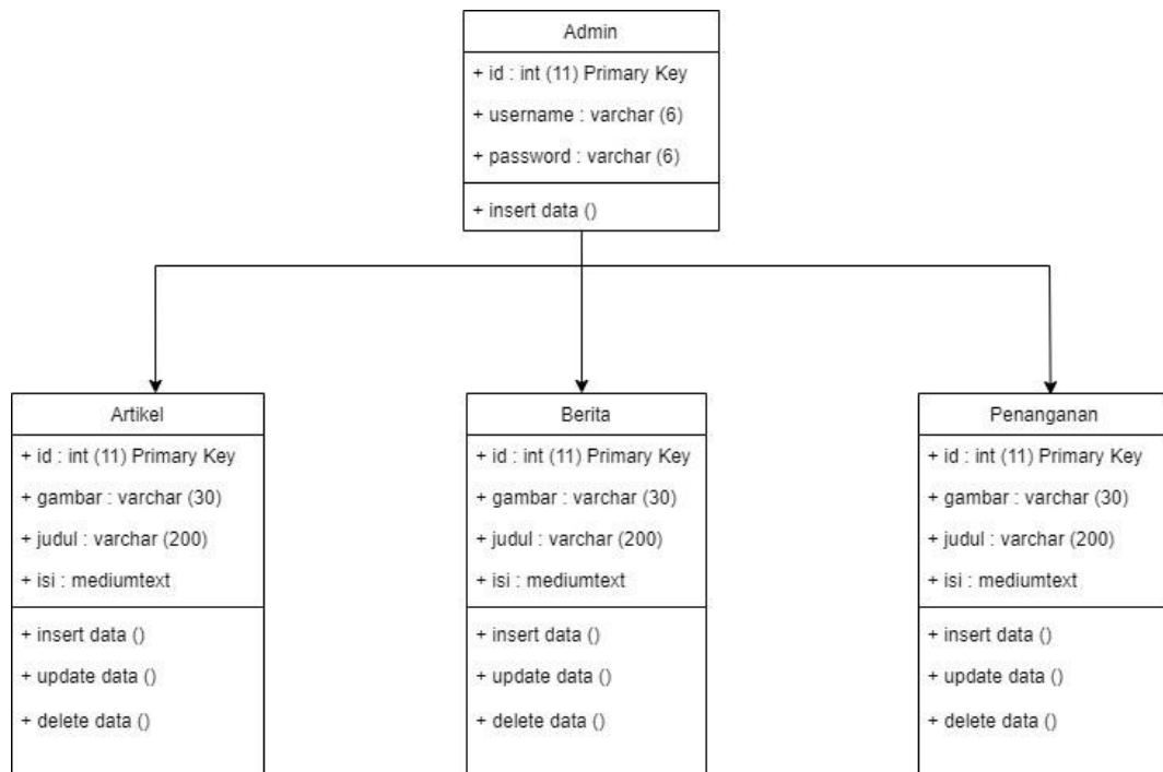
Gambar 8. Class Diagram
