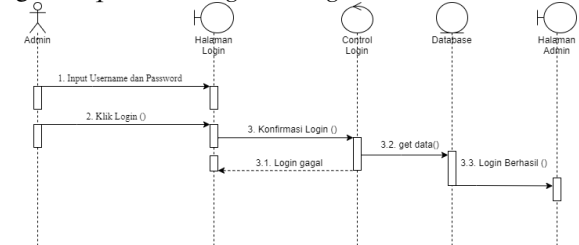
Gambar 12. Sequence Diagram Login
