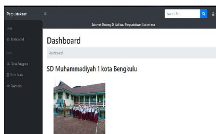
Gambar 2. Halaman Dashboard
