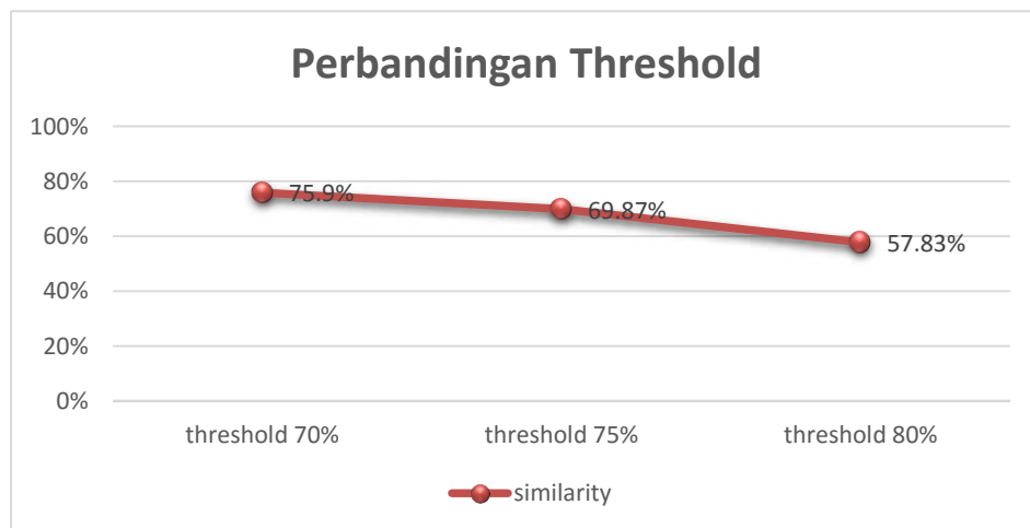
Gambar 2. Diagram similarity
