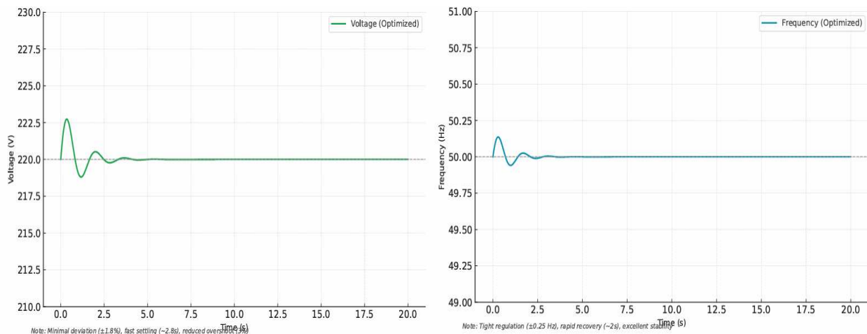
Figure 4. Voltage and Frequency Response under Optimized Control
