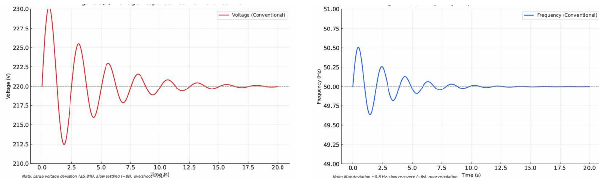
Figure 3. Voltage and frequency response
