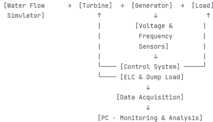
Figure 2. experimental setup block diagram
