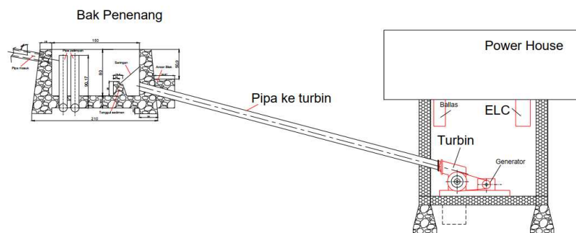
Figure 1. The micro-hydro powerplant layout
