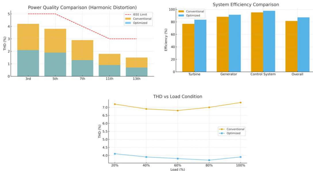
Figure 7. Power Quality Improvements
