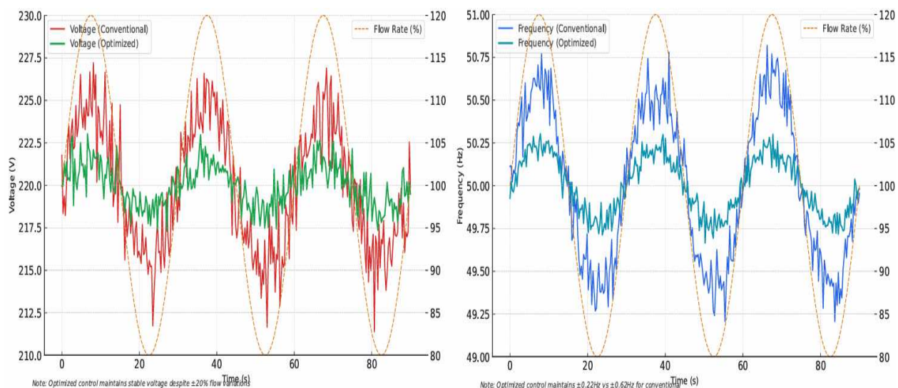
Figure 5. System Response to Water Flow Variations
