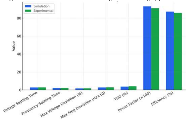
Figure 8. Simulation vs. Experimental Validation
