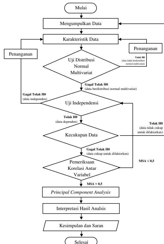
Gambar 1. Diagram Alir
