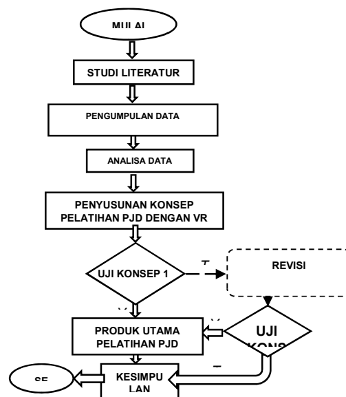
Gambar 3.3 Diagram Alir
