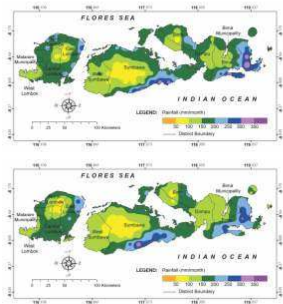
Figure 8. Annual mean monthly rainfall projection based on ECHAM5/MPI-OM for the periods 2050–2069 (top) and 2080–2099 (bottom)
