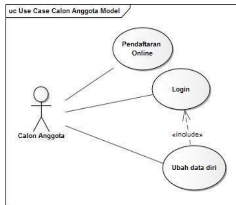
Gambar 2. Use Case Diagram Halaman Calon
