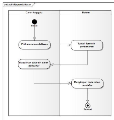
Gambar 5. Activity Diagram Halaman Pendaftaran
