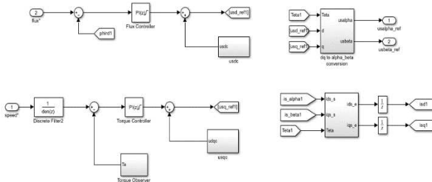
Gambar 8. Rangkaian vector control .
