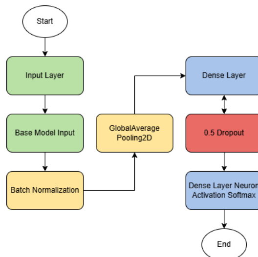
Gambar 6. Model Architecture
