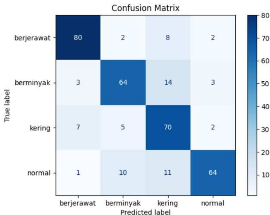
Gambar 14. Confusion Matrix of MobileNetV2
