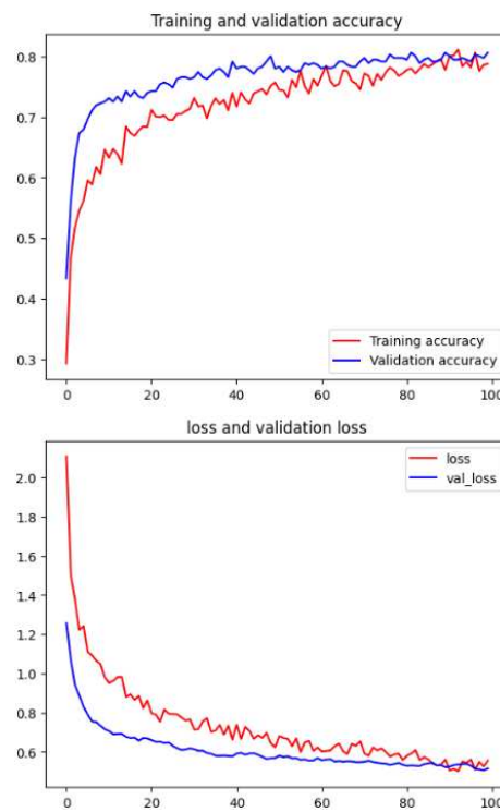
Gambar 11. Accuracy and Loss Curve for MobileNetV2
