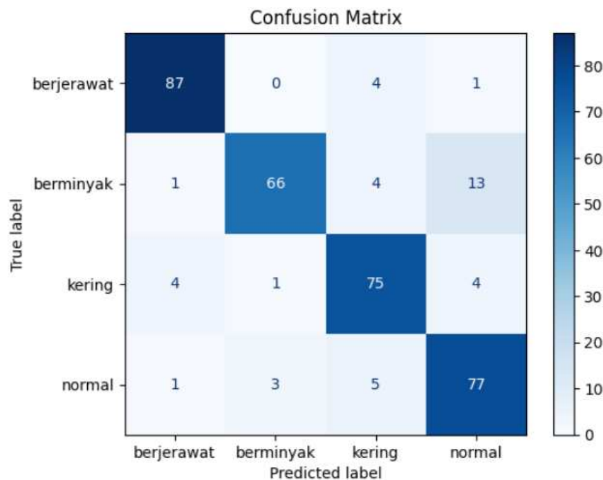
Gambar 13. Confusion Matrix of InceptionV3
