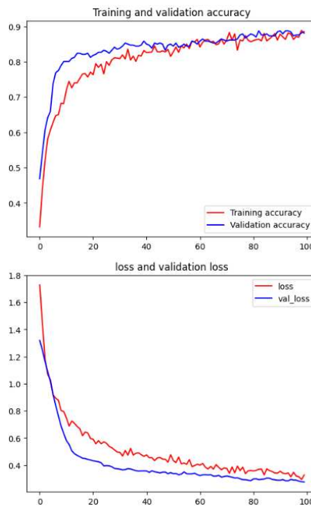
Gambar 9. Accuracy and Loss Curve for InceptionV3
