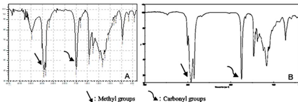
Figure 1. The IR spectrum of fungal lipids from N. surinamensis (A) and triacylglycerol from literature (B)
