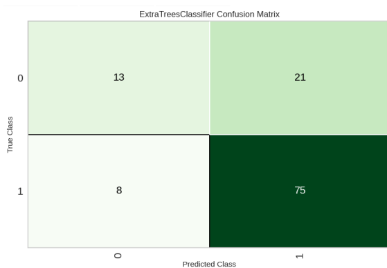
Gambar 4. Confusion matrix
