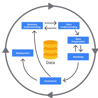
Gambar 1. Metode CRISP-DM
