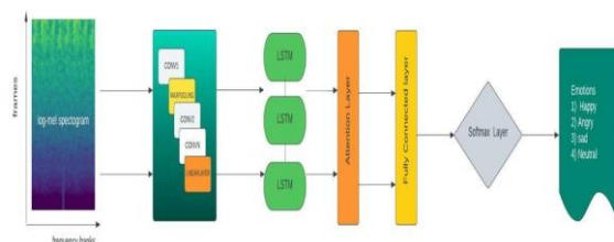
Fig. 1. ACRNN architecture
