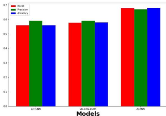
Fig 6. Comparison of Models and Their Evaluation Metrics
