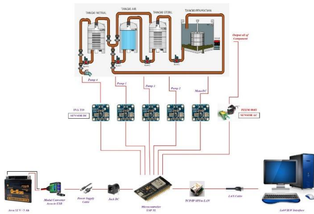
Gambar 8. wiring monitoring
