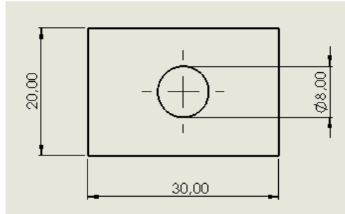
Figure 5. Plastic Insulator
