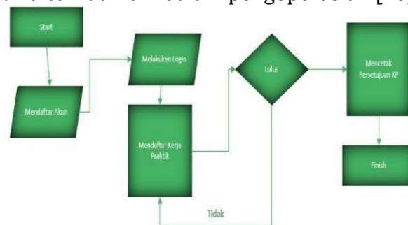
Gambar 3.2 Flowchart
