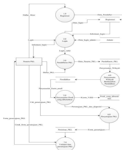
Gambar 3.5 Data Flow Diagram
