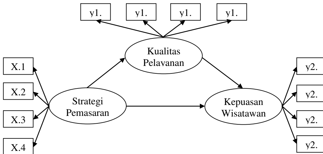
Gambar 1. Model Struktur Penelitian
