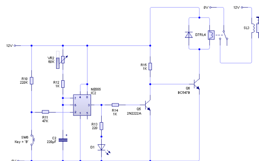
Gambar 9. Selenoid Valve
