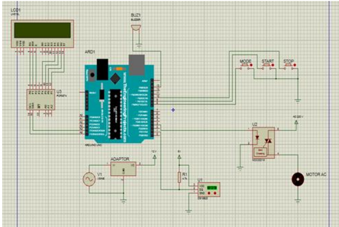
Figure 2 Diagram Circuit
