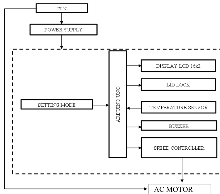
Figure 3 Block Diagram
