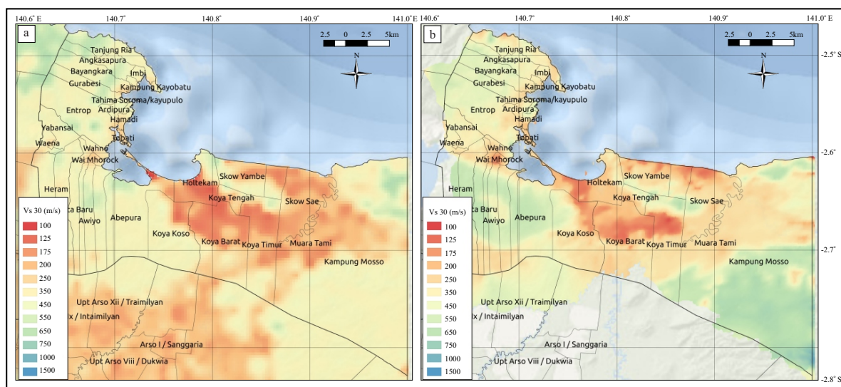
Figure 7: Maps of V_{s30} derived from (a) engineering geomorphology and (b) HVSR microtremor inversion. Both maps show the similar pattern. However, the engineering geomorphology V_{s30} tends to have lower values except in the area in the middle of the map and the north coast between the longitude of 140.8^{\circ} – 140.9^{\circ} .
