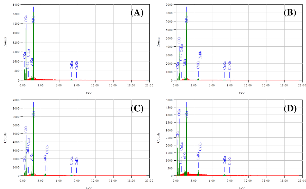
Figure 5. Elemental composition of catalysts: (A) HY, (B) 5CaCO 3 /HY, (C) 10CaCO 3 /HY, and (D) 20CaCO 3 /H.
