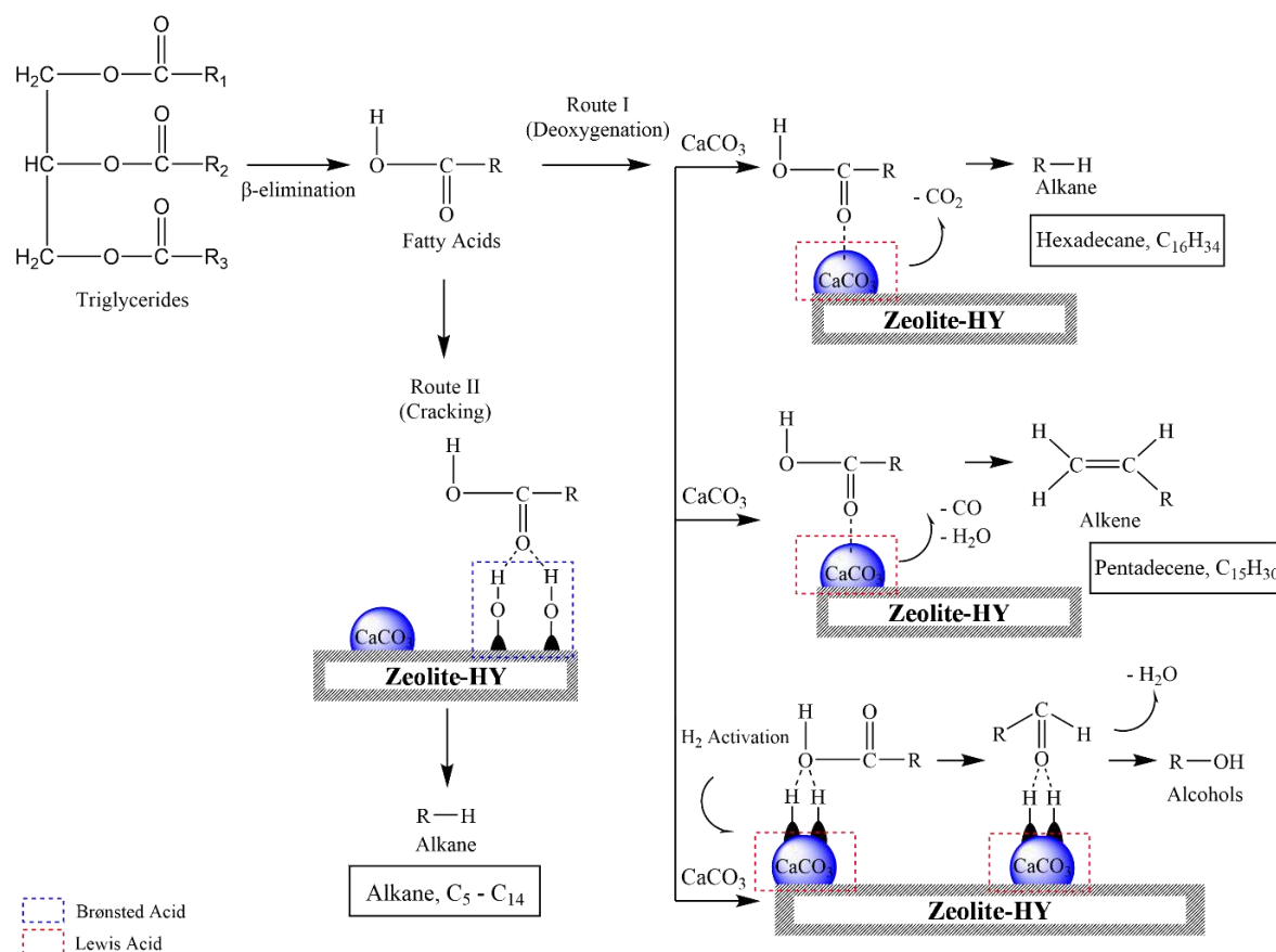
Figure 10. Proposed reaction mechanisms of catalytic cracking-deoxygenation over CaCO 3 /HY catalysts.
