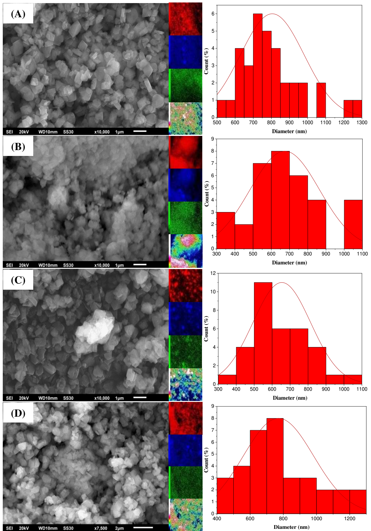
Figure 4. SEM characterization results of catalysts: (A) HY, (B) 5\text{CaCO}_3/\text{HY} , (C) 10\text{CaCO}_3/\text{HY} , dan (D) 20\text{CaCO}_3/\text{HY} .
