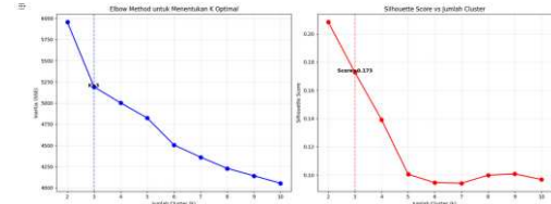
Figure 7. Elbow and Silhouette Score for Determining K
