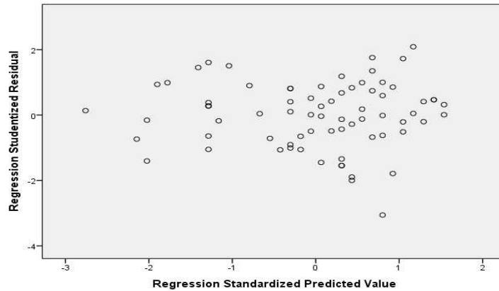
Gambar 1 Hasil Heteroskedastisitas-Scatterplot
