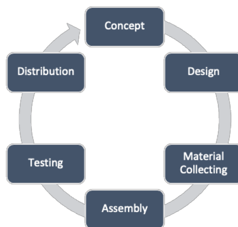
Gambar 1. Metode MDLC
