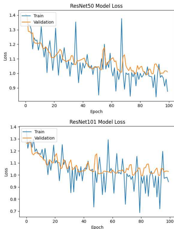
Figure 5. Model loss before image preprocessing. Top: ResNet50, bottom: ResNet101
