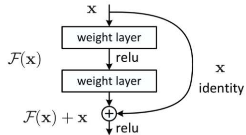
Figure 4. Residual learning unit of ResNet.
