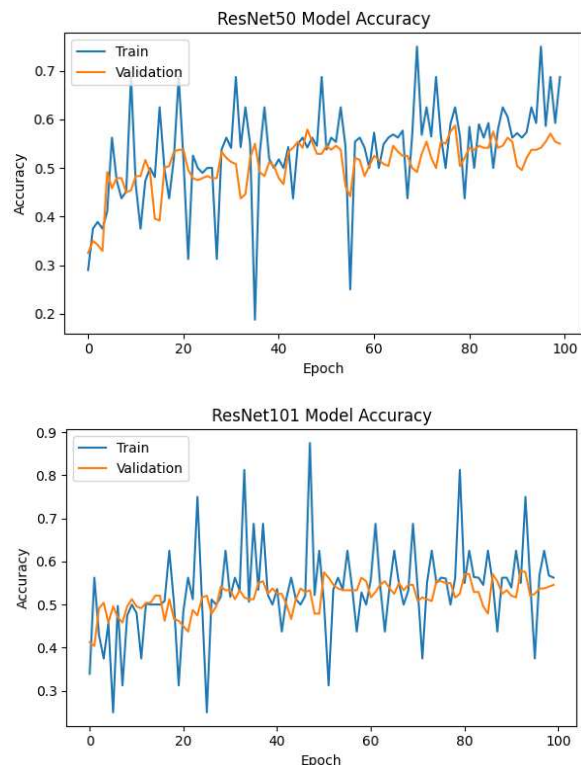
Figure 6. Model accuracy before image preprocessing. Top: ResNet50, bottom: ResNet101
