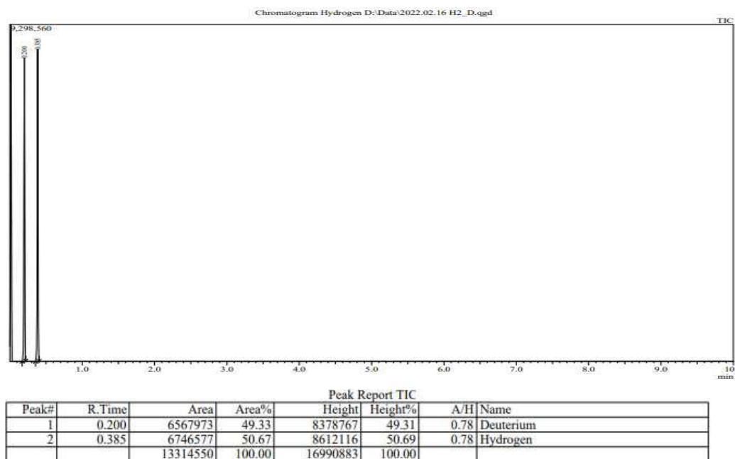
Gambar 3.4 hasil gas Chromatography-Mass Spectrometry (GC-MS)
