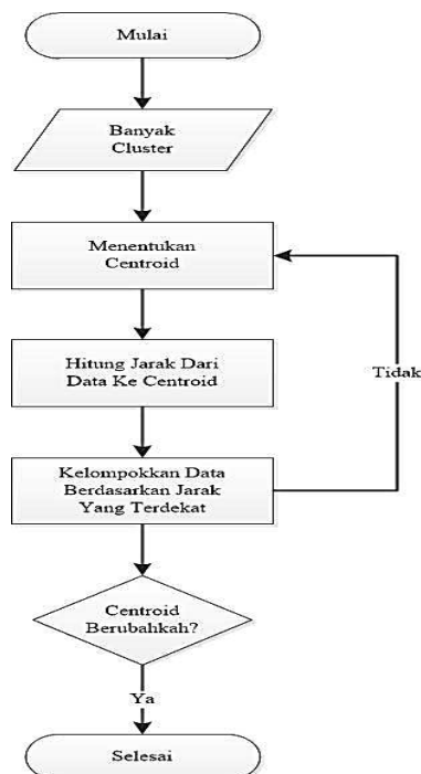
Figure 2. K-Means Algorithm Flowchart
