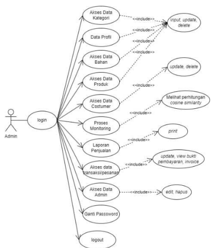
Gambar 4. 3 Use Case Diagram Admin
