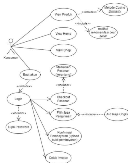
Gambar 4. 1. Use Case Diagram Konsumen
