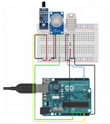
Gambar 2. Rangkaian sensor flame, DHT22, sensor mq-2
