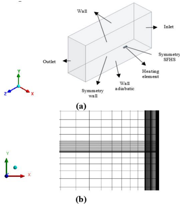
Figure 2. (a) Computational Domain and Boundary Condition Determination, (b) Tetrahedral Grid Structure.
