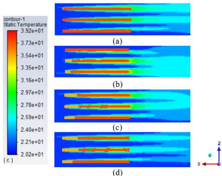
Figure 9. (a, b, c, and d) SFHS Temperature Contours t = 3 mm X-Z Plane Direction Height Y = 5 mm from Heating Element at v = 4 m/s, 6 m/s, 8 m/s, and 10 m/s.
