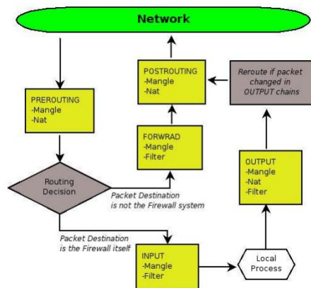
Gambar Diagram Iptables
