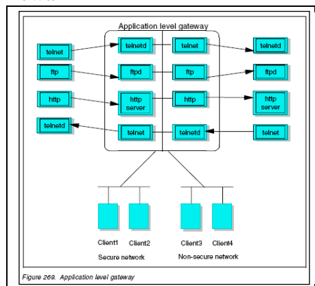
Figure 269. Application level gateway
