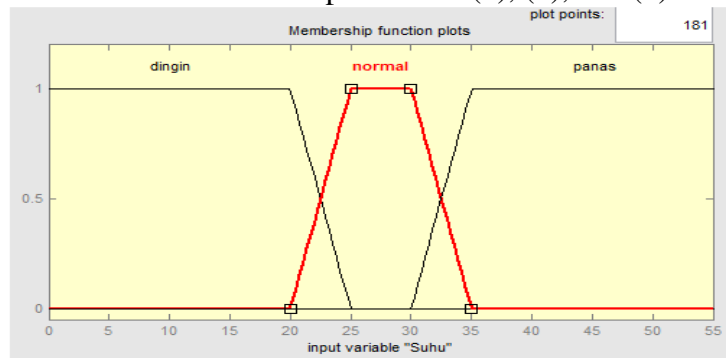
Gambar 3. Himpunan Fuzzy Variabel Suhu
