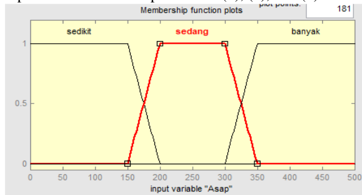
Gambar 4. Himpunan Fuzzy Variabel Asap
