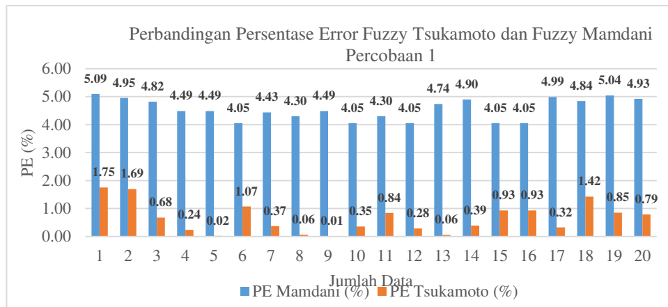
Gambar 8. Perbandingan Persentase Error Fuzzy Tsukamoto dan Fuzzy Mamdani
