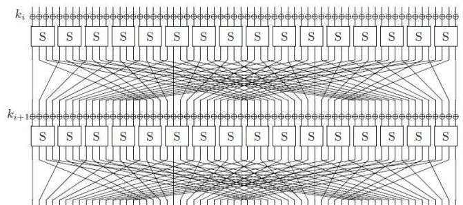
Gambar 7 Skema operasi SPN [26]
