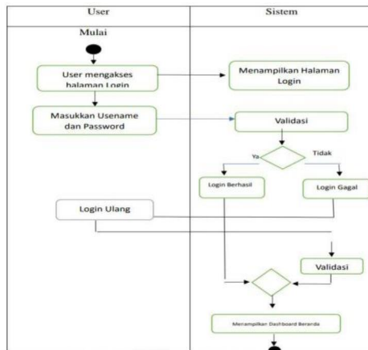
Gambar 11. Activity Diagram Login
