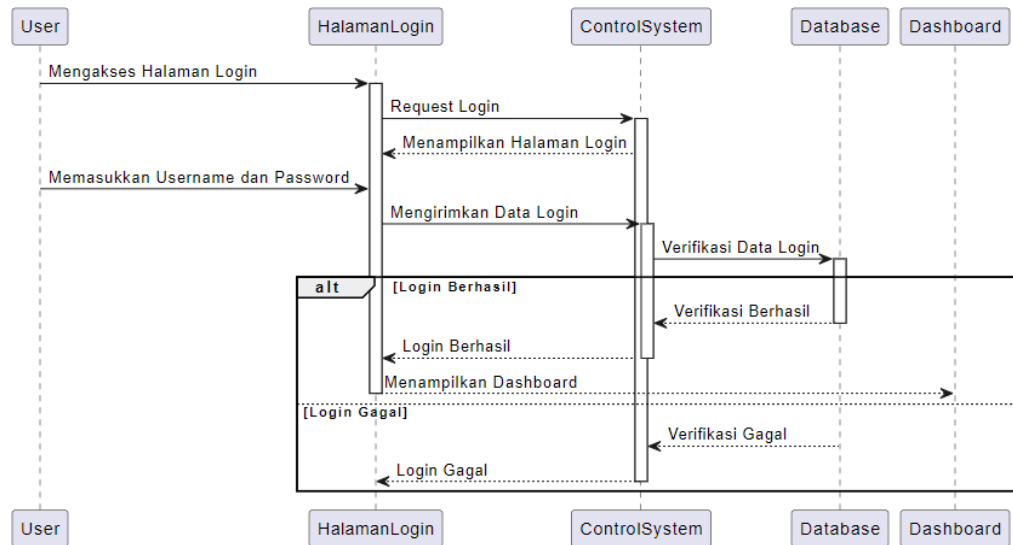
Gambar 12. Sequence Diagram Login
