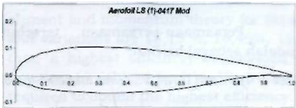
Gambar 3-1: Aerofoil LS (1)-0417
