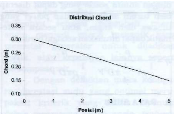
Gambar 3-2: Grafik Distribusi chord sudu
