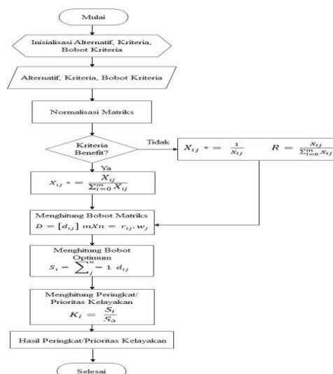
Gambar 1. Flowchart Metode Additive Ratio Assesment (ARAS)
