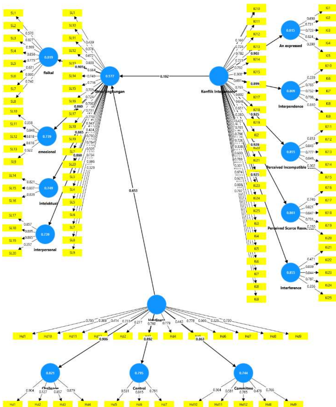
Gambar 1 Output PLS Algorithm Model Keseluruhan
