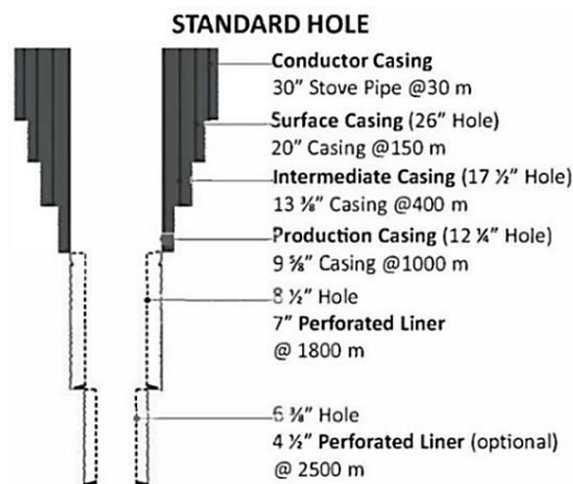
Gambar 5 Well Geometry of Standart Hole
