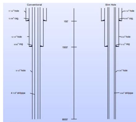
Gambar 3 Well Geometry of Slimehole & Conventional
