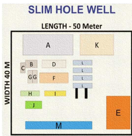
Gambar 7. Area Slim Hole Well
