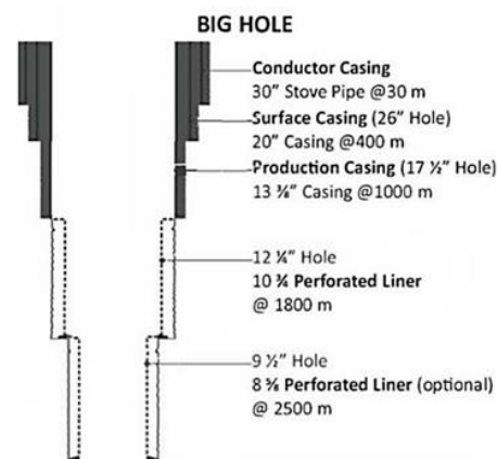
Gambar 4 Well Geometry of Big Hole
