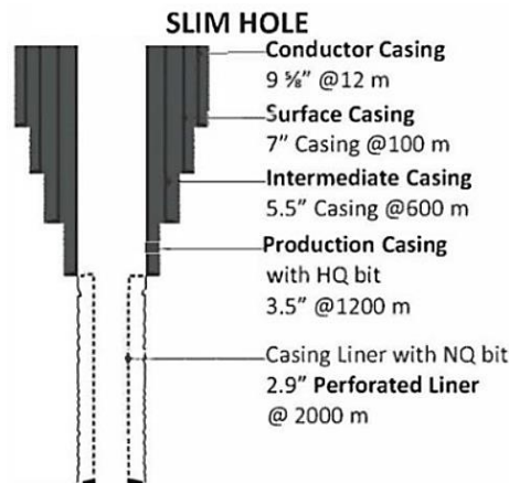
Gambar 6 Well Geometry of Slim Hole
