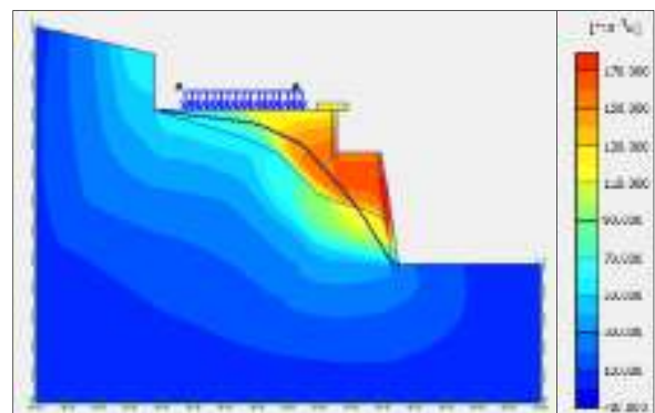
Gambar 10. Horizontal displacement (horizontal disp.= 179.23 \times 10^{-3} m)
