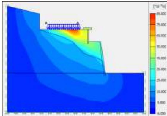
Gambar 6. Total Displacement (total disp.= 80.66 \times 10^{-3} m)
