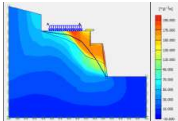
Gambar 9. Total Displacement (Total disp.= 189.95 \times 10^{-3} m)
