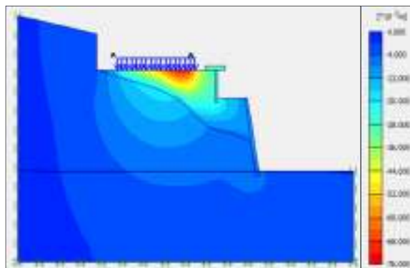
Gambar 7. Horizontal Displacement (Horizontal disp.= 45.78 \times 10^{-3} m)
