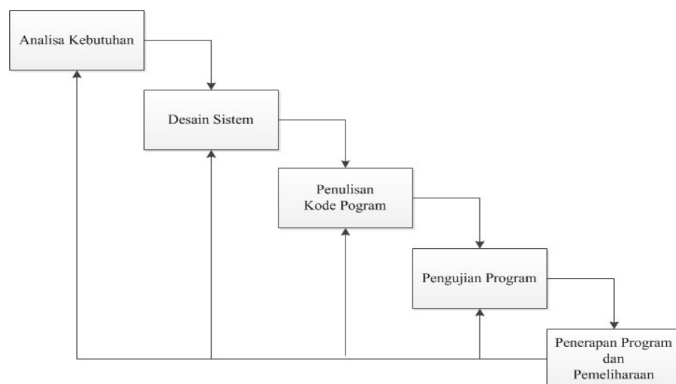
Gambar 1 Tahapan Waterfall
