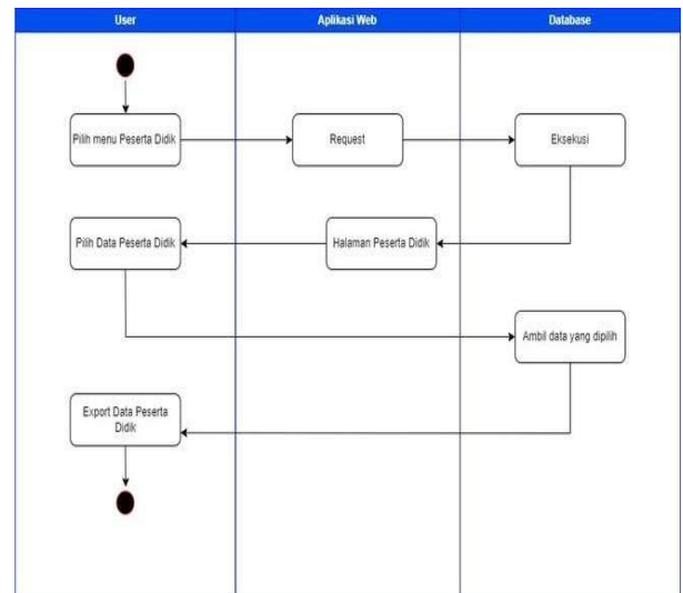
Gambar 8 Activity Diagram Menu Peserta Didik
