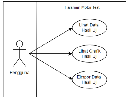
Gambar 2. Use Case Diagram Halaman Motor Test
